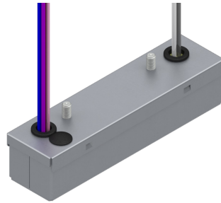
Bottom Leads with Studs: "-S" Suffix L 103.5 * W 26.2 * H 23.85 mm (L 4.07 * W 1.03 * H 0.94 in.)
