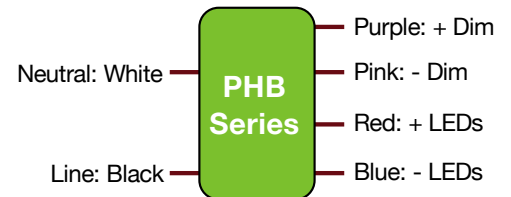
Wiring Diagram
