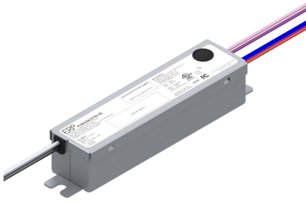
Side Leads L 103.5 * W 26.2 * H 23.85 mm (L 4.07 * W 1.03 * H 0.94 in.)
