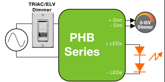
Application Diagram
