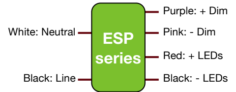
Wiring Diagram
